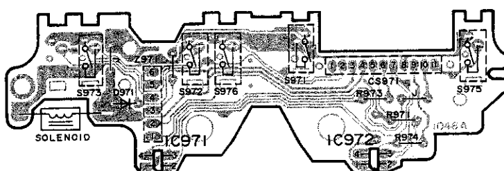
D MECHANISM P.C.B. (REP1656A)
