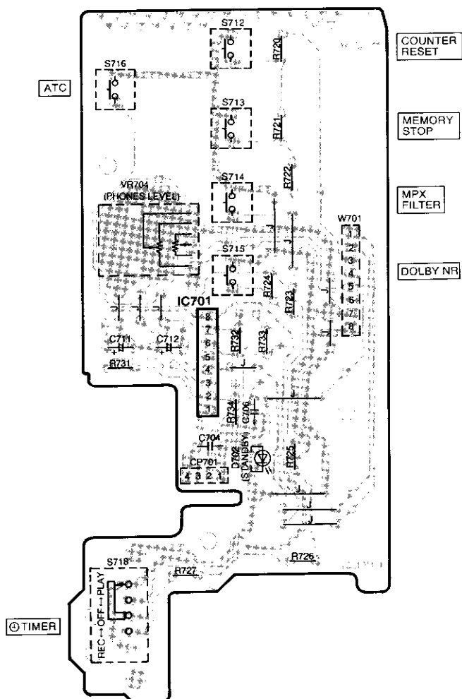
F OPERATION P.C.B. (REP2285A-S)
