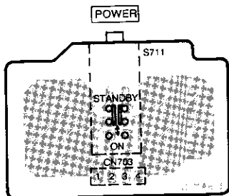
B POWER SWITCH P.C.B. (REP2285A-S)
