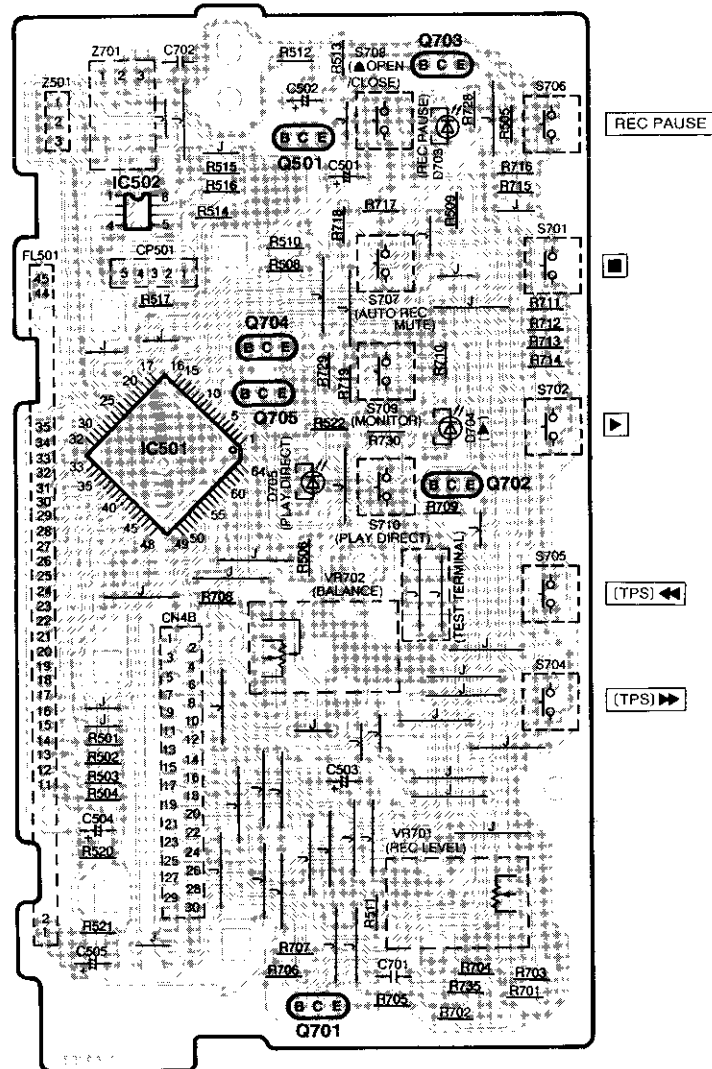
H FL P.C.B. (REP2285A-S)
