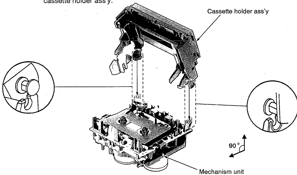
Mechanism unit
