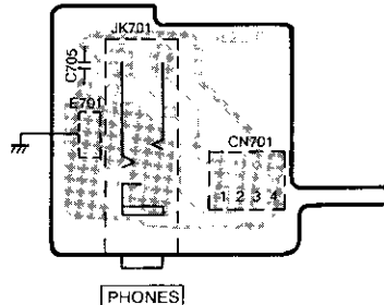
E HEADPHONES JACK P.C.B. (REP2285A-S)
