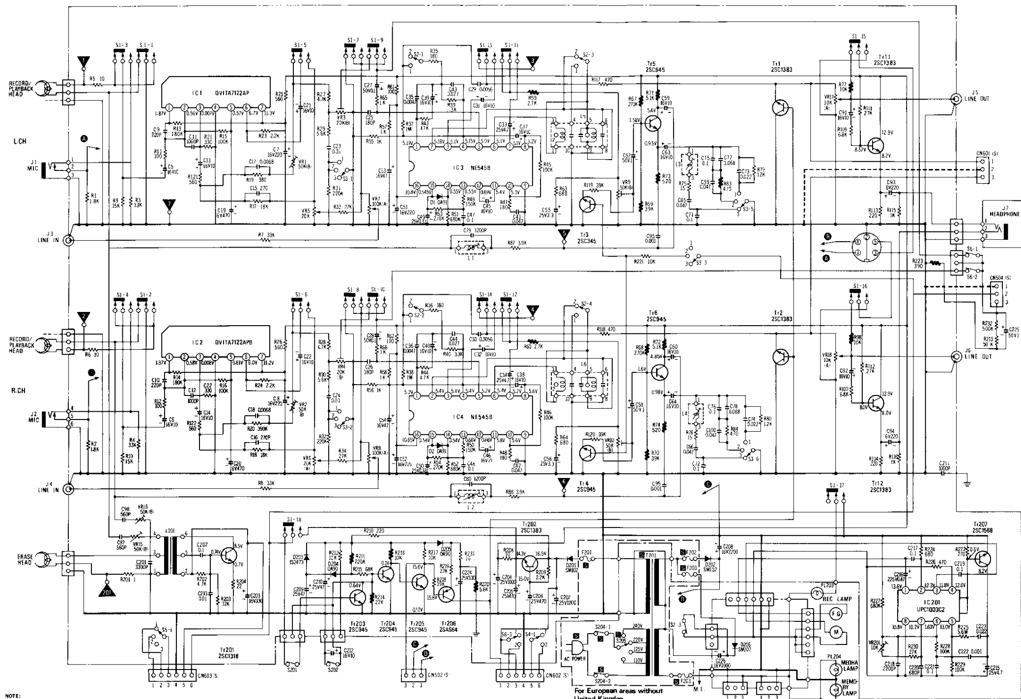
IC1, 2 QV1A7122AP
