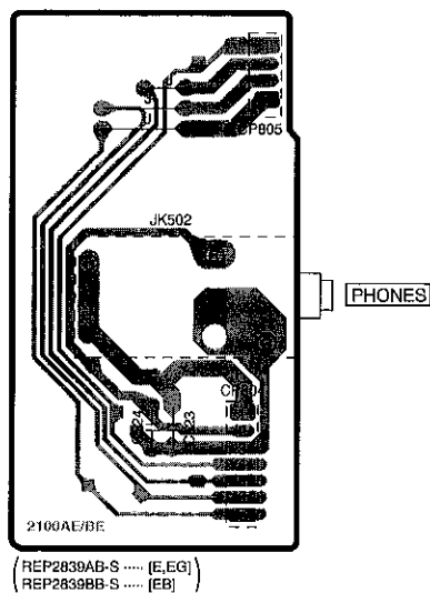
E HEADPHONES JACK P.C.B.
