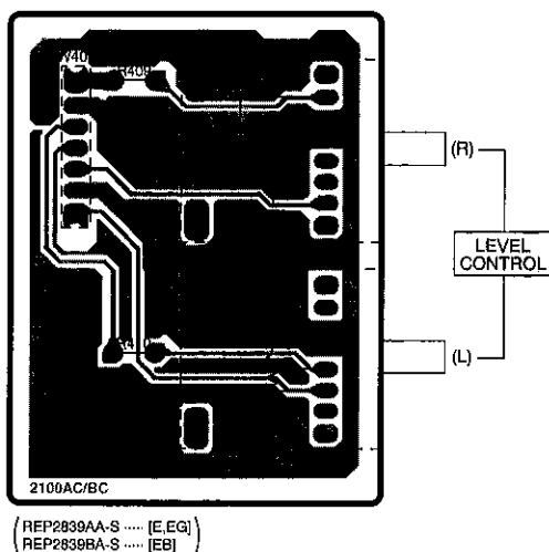
B LEVEL CONTROL P.C.B.
