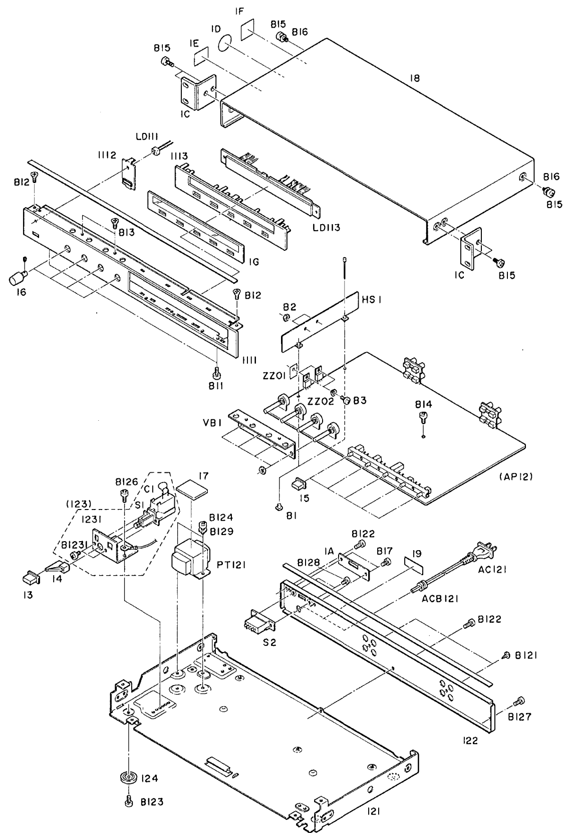
EXPLODED VIEW
