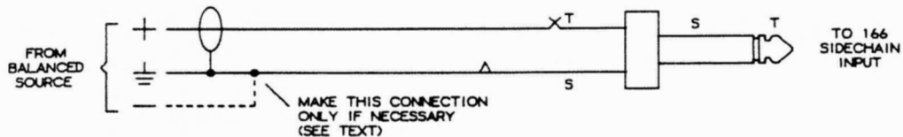
Figure 7b: Balanced source
