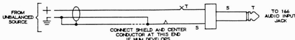
Figure 3b: Same, mono plug
