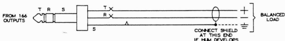
Figure 4: Balanced ins and outs, dual-conductor shielded cable, stereo plug
