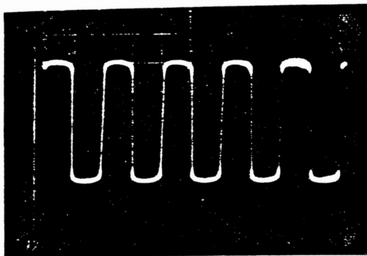
Figure D. Peakstop circuit limiting +20 dBv signal to approx 4v P-P.
