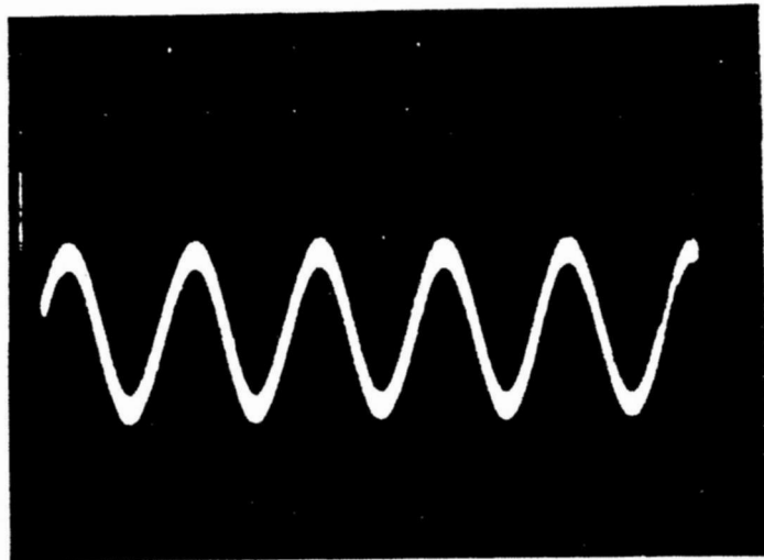
Figure B. TP1(TP5) After Adjusting R34(R154) for peaks at 0 vdc. (1mV/div, DC coupled)
