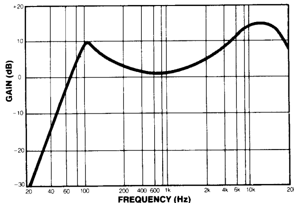
402-E Active Equalizer gain characteristics.
